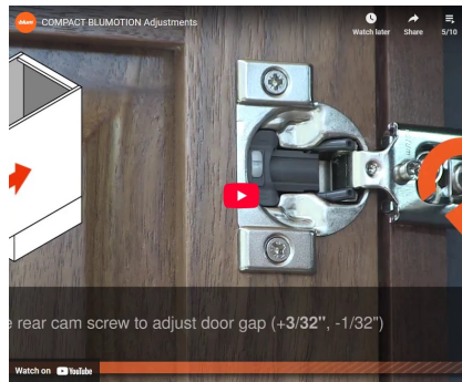
Compact Blumotion Adjustments
